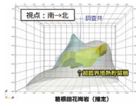
Fig. 1 Supercritical geothermal system at a Japanese geothermal site
