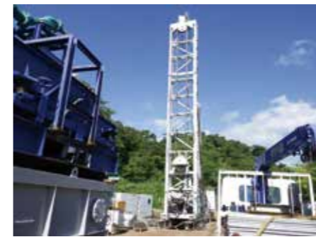
Fig. 4 Exploration drilling of hot spring in Fukushima
