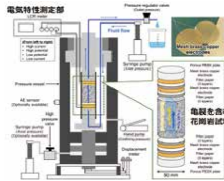
Fig. 3 Rock hydraulic, mechanical, and electrical properties simultaneous measurement system
