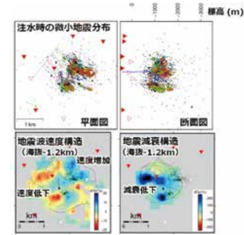
Fig. 5 Distribution of velocity and attenuation around microearthquake hypocenters in a geothermal area
