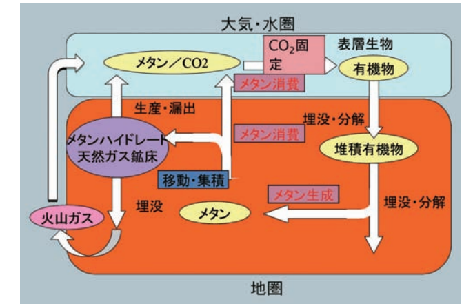
Fig.3 Global material circulation of greenhouse gases, methane and carbon dioxide, in marine and geo-environment.
