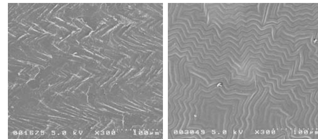
Fig.3 A SEM photo of snail shell surface (left), and created micro-wrinkle (right).
