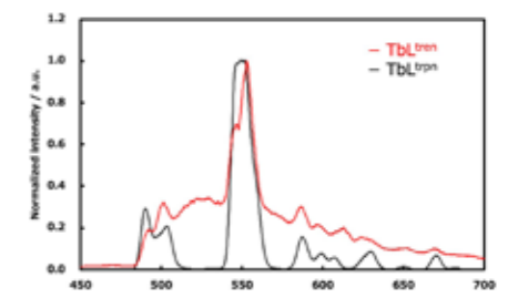
Fig.6 Emission spectra of TbL tren and TbL trpn .
