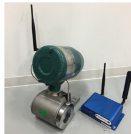
Fig.4 Remote monitoring system of hot springs for coexistence of geothermal power generation and hot springs
