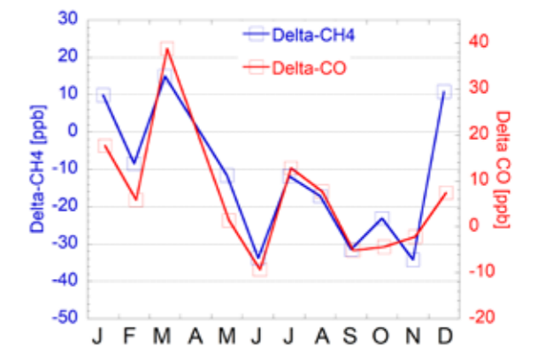
Fig.4 Seasonal variations in vertical gradient of CH 4 and CO over Bangkok.
