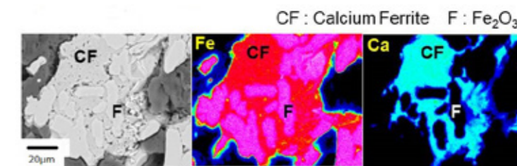
Fig.3 Mineral formation in sintered pellet.
