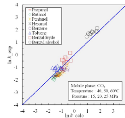
Fig.4 Results of prediction of retention time with separated chemicals on supercritical fluid chromatography.
