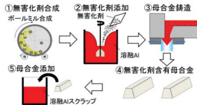
Fig. 1 Fabrication of intermetallic compound modifier Process flowchart
