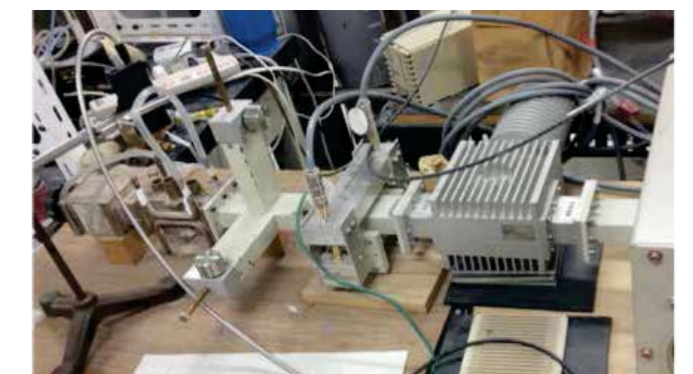
Fig.5 Microwave single mode applicator of 5.8GHz for rapid synthesis of ZrB 2 ceramics.
