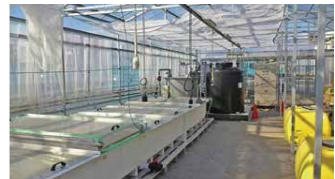
Fig.3 The pilot plant for culturing microalgae at Minamigamo sewage plant (Task 2)
