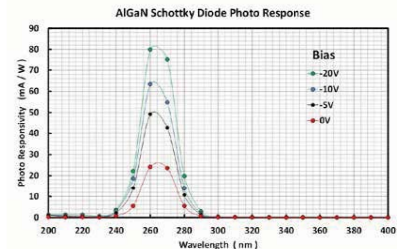
Fig.4 Photo responsivity of the AlGaN photodetector.
