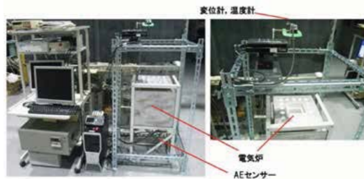
Fig.2 Evaluation system for deformation/temperature/AE of SOFC planer cell.
