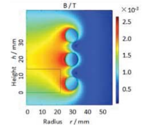
Fig.4 Simulated magnetic field distribution on a cross section of water-cooling coil (circles) and specimen with imposition RF (400kHz) EM field.
