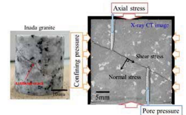
Fig.5 Granite specimen for slip experiment.
