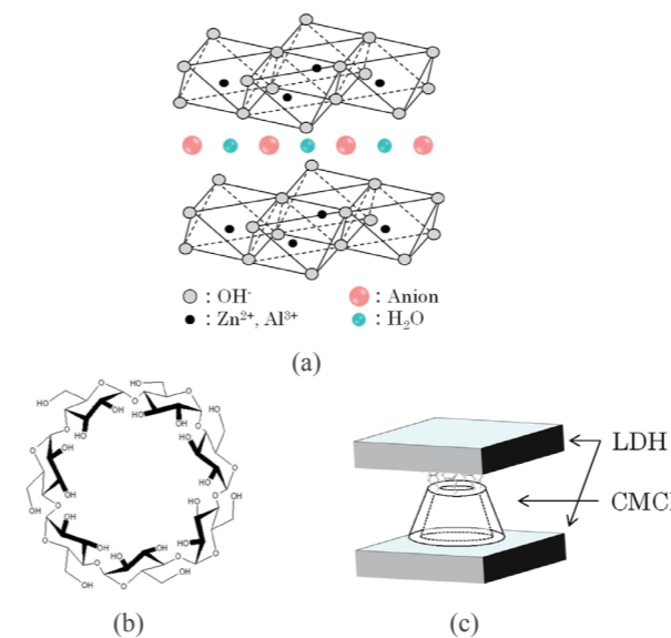
Fig.3 The structure of (a) Zn-Al LDH, (b) beta-cyclodextrin, and (c) CMCD-Zn-Al LDH
