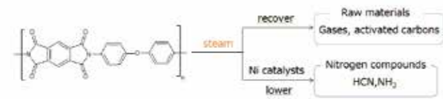
Fig.1 Scheme of steam pyrolysis of polyimide
