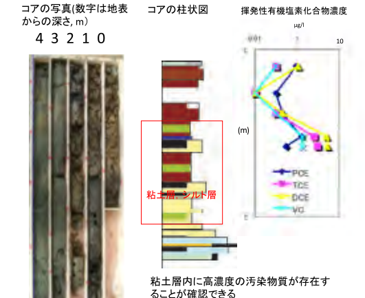
Fig.3 Distribution of contaminants in impermeable strata at a contaminated site.
