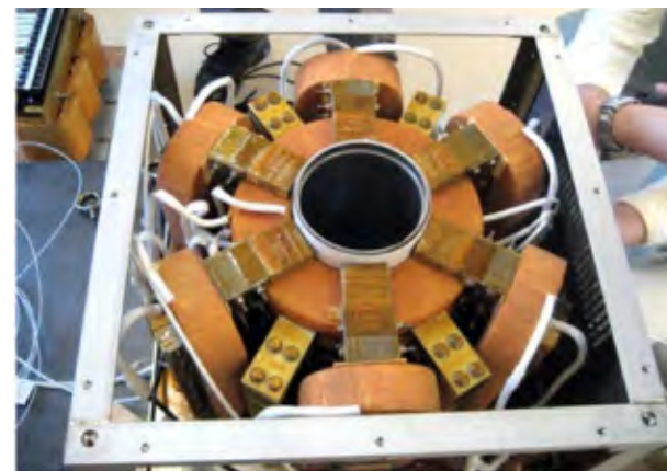
Fig.1 Double-Axis-Electromagnetic Stirrer
