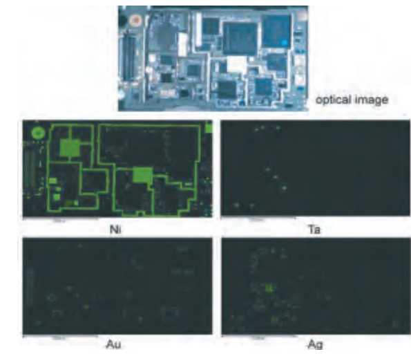
Elements mapping of PCB from mobile phone using micro-XRF instrument
